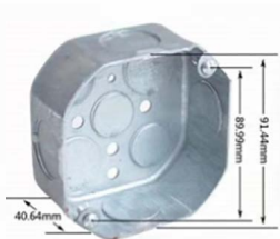
Octagon Box
